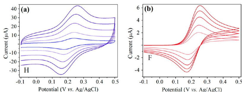
Figure 4. CV responses obtained using (a) honeycomb (H) and (b) flat (F) BDD electrodes for the ferri/ferrocyanide redox reaction taken at different scan rates ( 0.010, 0.025, 0.050, 0.075, and 0.1 \text{ V s}^{-1} ).
